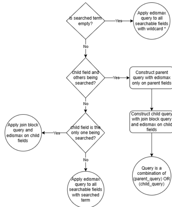
Image 4: Search route query building workflow.
